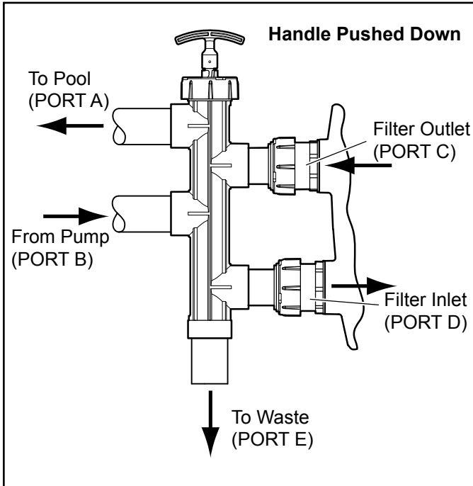
Figure 5. SVLV2 Plumbing Configuration for DEL, DEV and JS Series Filters - Filtration Mode
