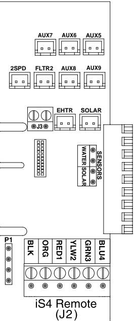
i10D, Dual Equip. (P/N 521915)
