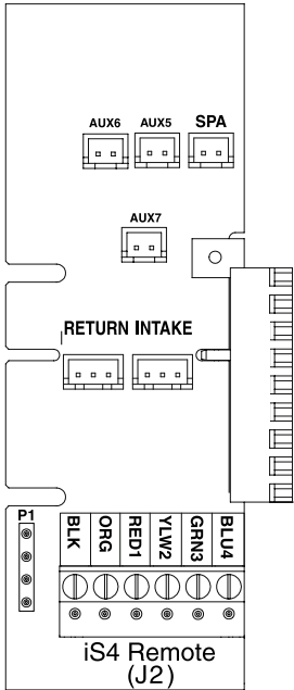
i8PS, Shared Equipment (P/N 521913)
