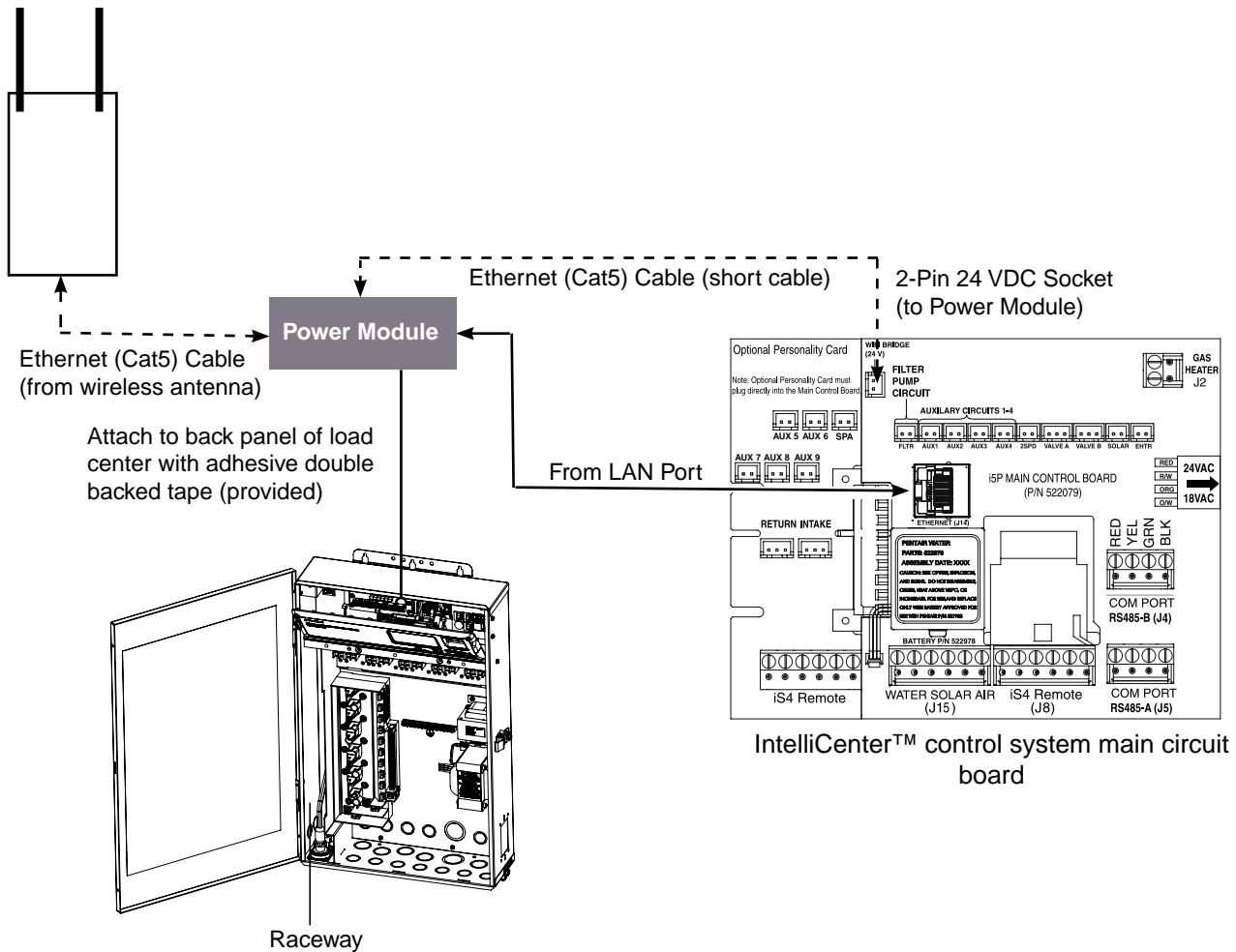
IntelliCenter™ Control System Load Center
