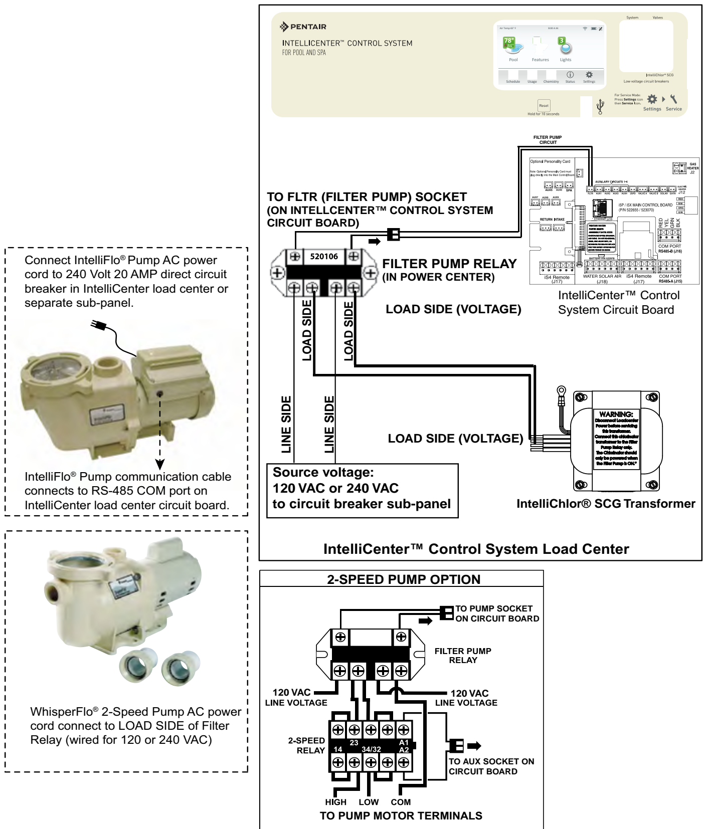
IntelliCenter™ Control System Load Center - IntelliChlor® SCG Connection Diagram
