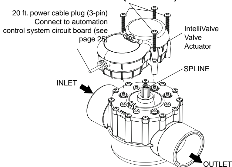
IntelliValve Valve Actuator Mounted on a 2-Port Valve assembly
