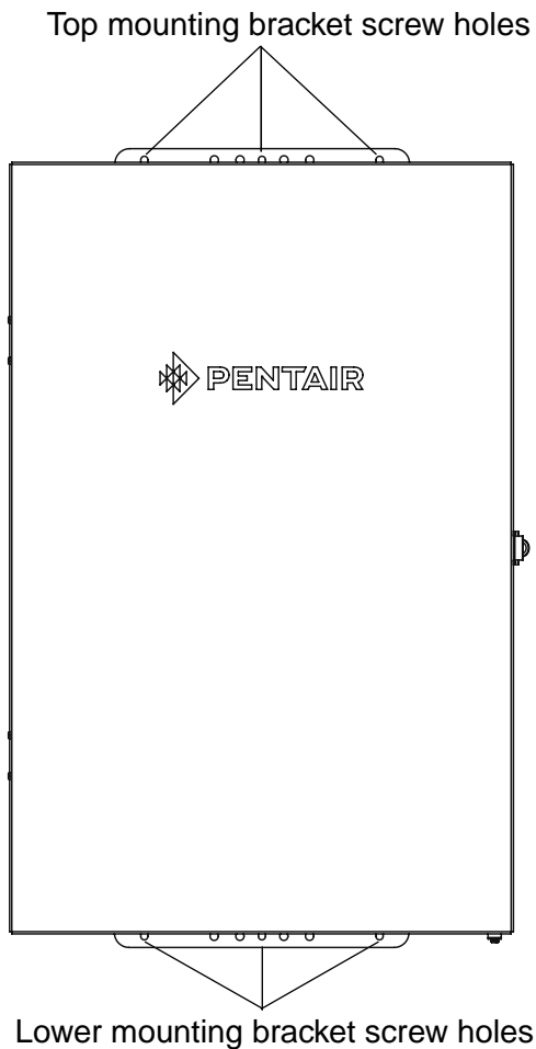
IntelliCenter™ Control System Load Center (26" H x 17" W x 5¼" D)
