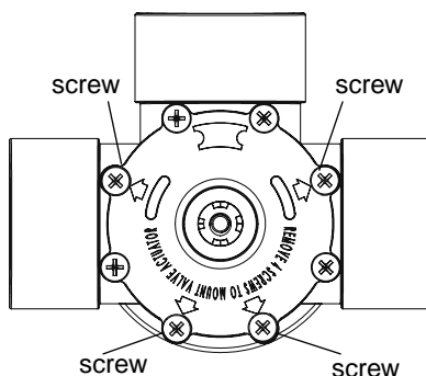
3-Way Valve Assembly
