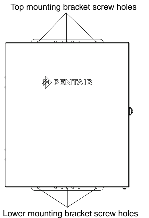
IntelliCenter Control System Power Center (20" H x 17" W x 5¼" D)
