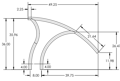
DR-D3D Deck to Deck Return Stair Rail
