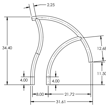
DR-G3DE Grab Rail - 24" height
