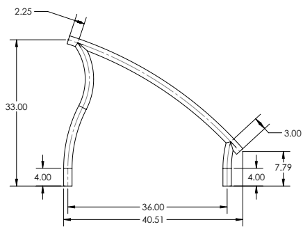
DR-D2D3 Deck to Deck Stair Handrail (pair)
