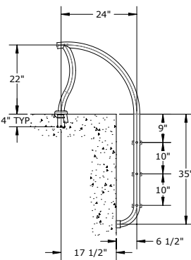
DR-D2D3 Deck to Deck Stair Handrail (pair)
