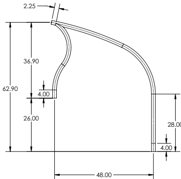
DR-D2S Deck to Stair Handrail
