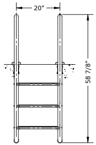
Designer 3 Tread Ladder
